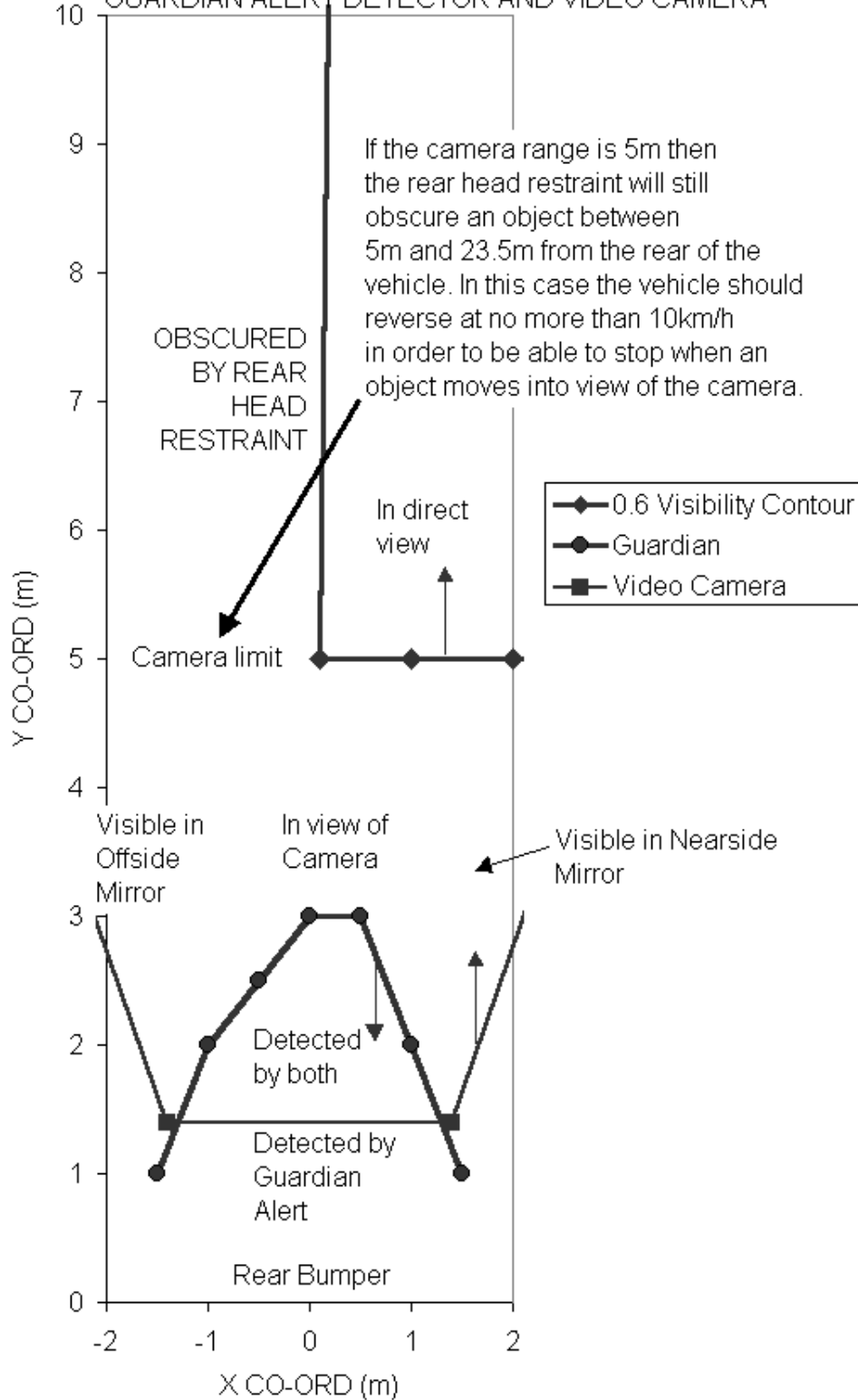
Figure 2. Performance of combined system - proximity sensor and video camera.
