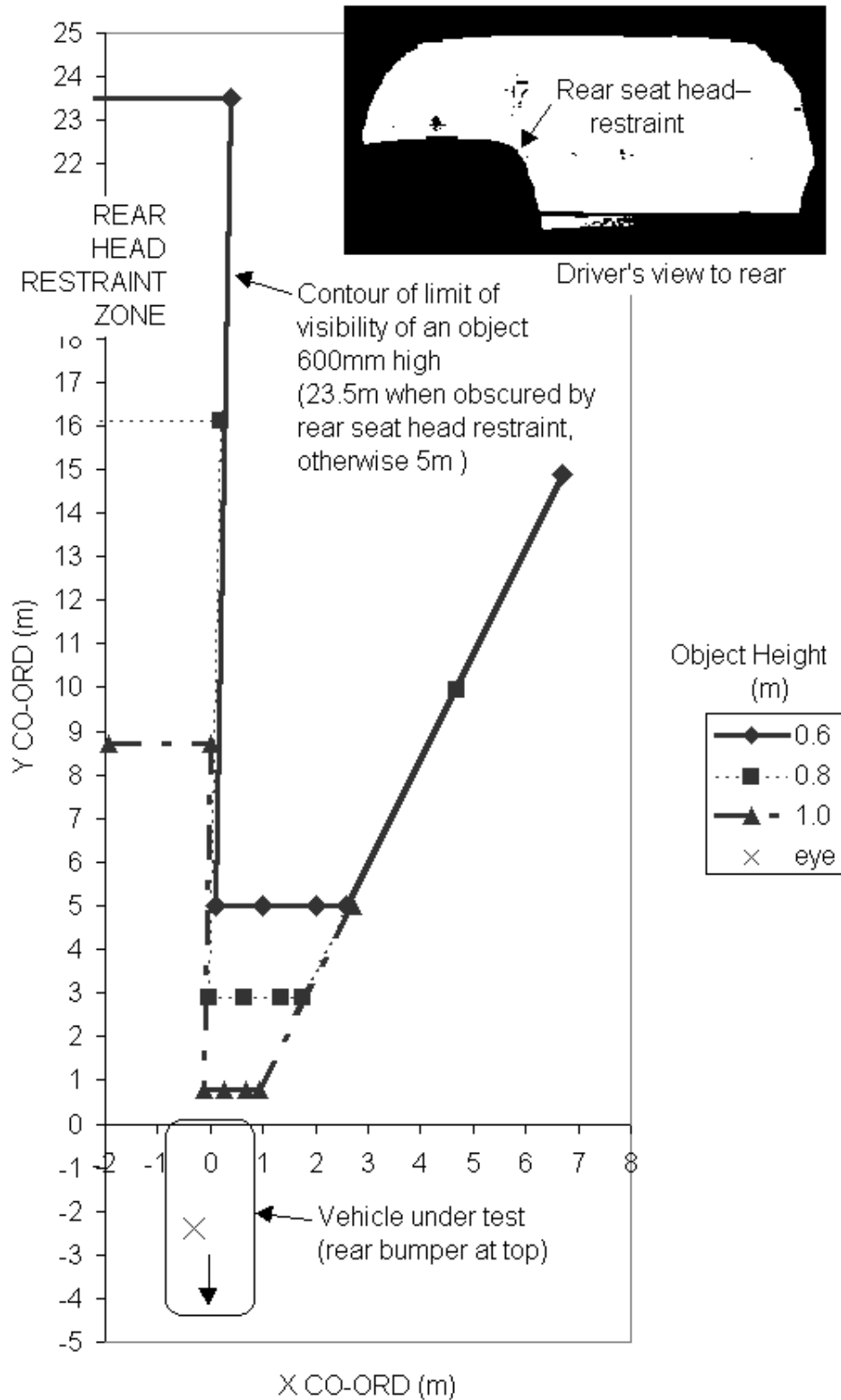
Figure 1. Rearward field of view for a Honda Odyssey passenger van.
