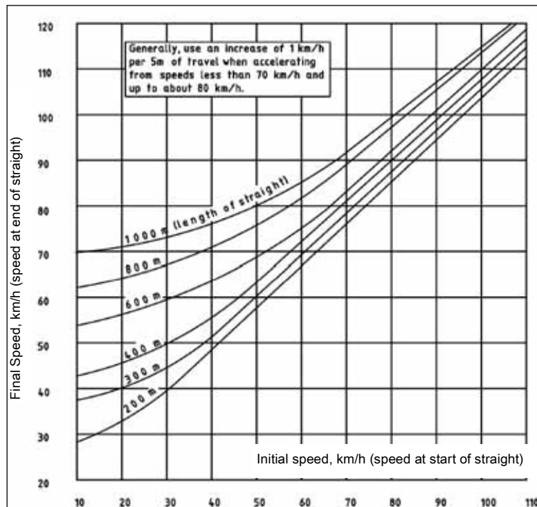
Figure 2. Acceleration on straights (source: Austroads, 2009)
