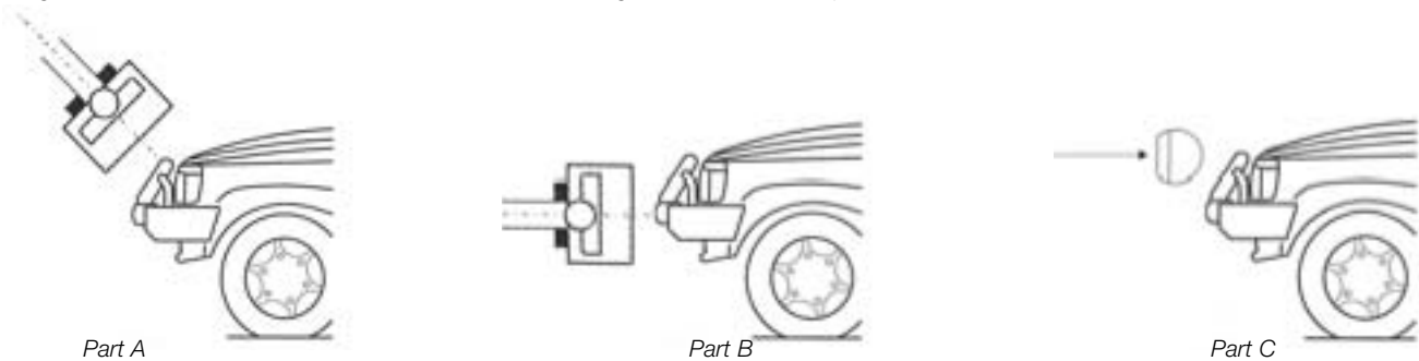
Figure 1 Schematic of Part A, Part B and Part C tests, using the EEVC WG17 impactors
