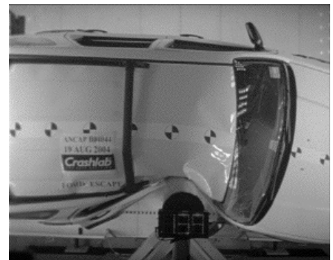
Figure 3. Pole crash test
